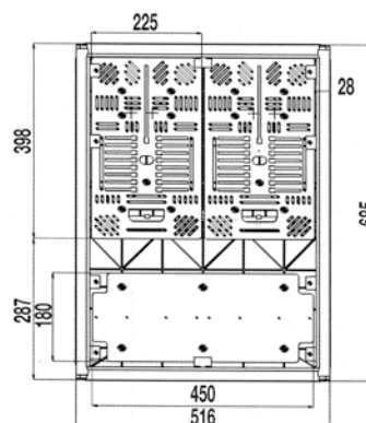
Front view without doors
