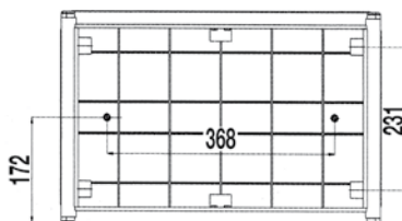
Front view without doors
