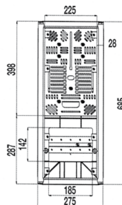
Front view without door
